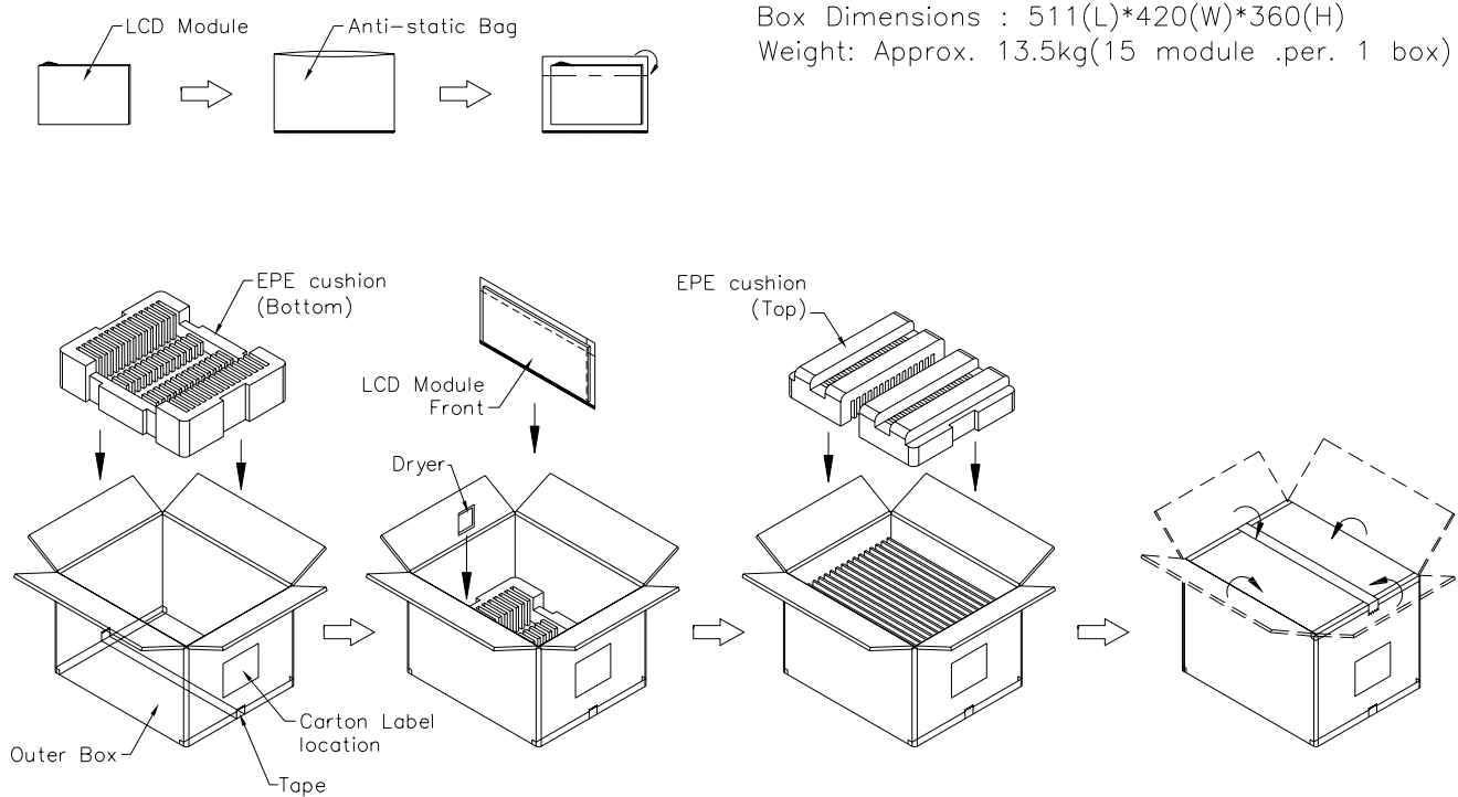
Figure. 9-1 Packing method
