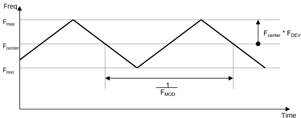
< Spread Spectrum >
