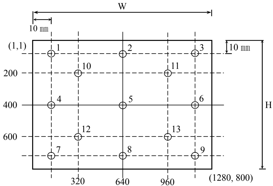
Fig.1 measuring points
