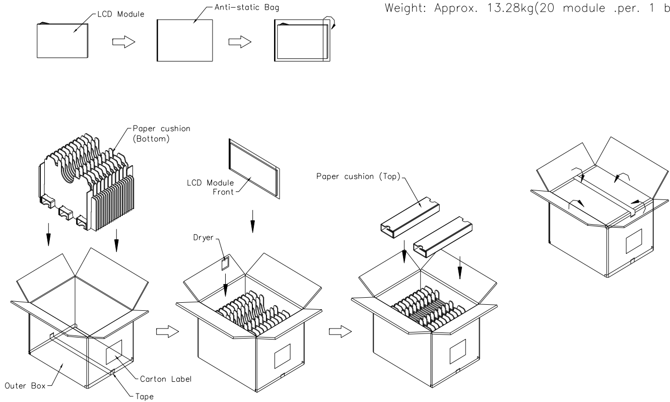
Figure. 9-1 Packing method
