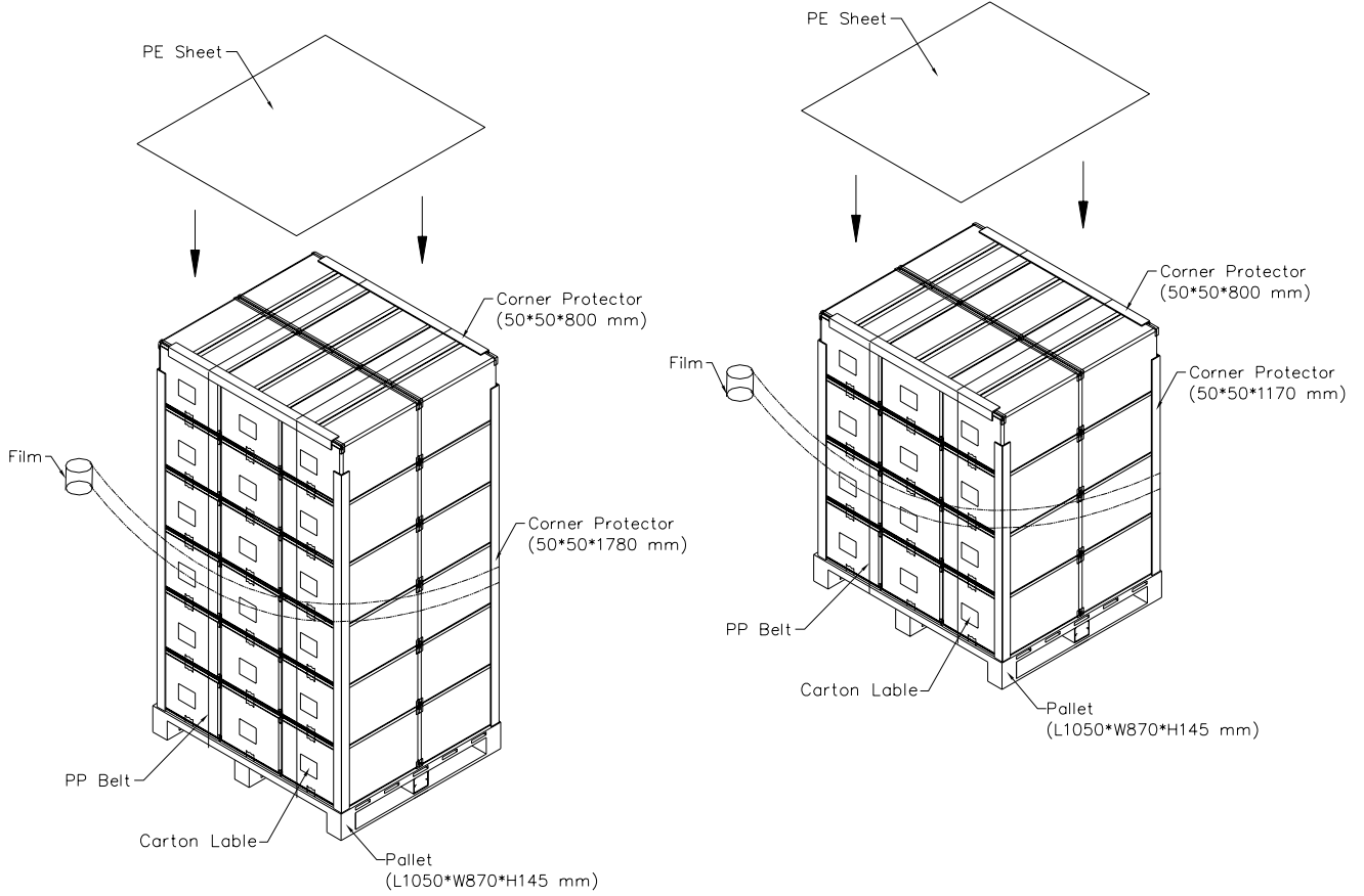
Figure. 10-2 Packing method
