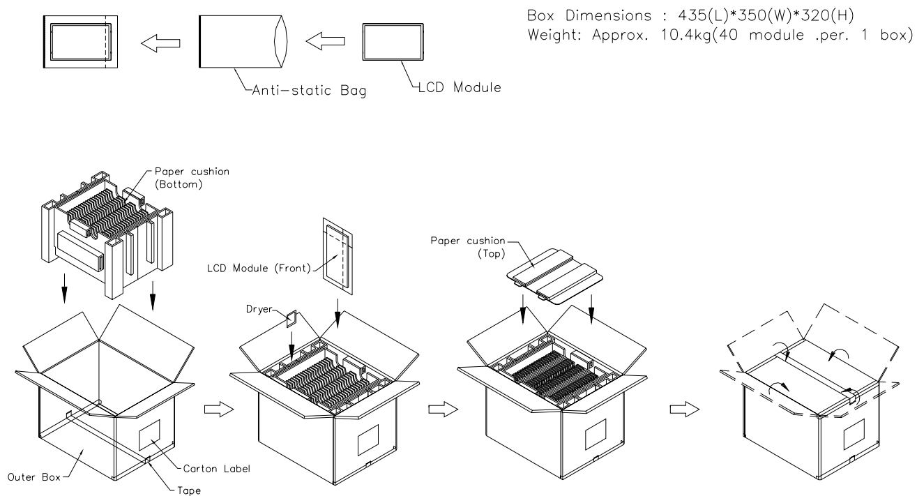
Figure. 10-1 Packing method
